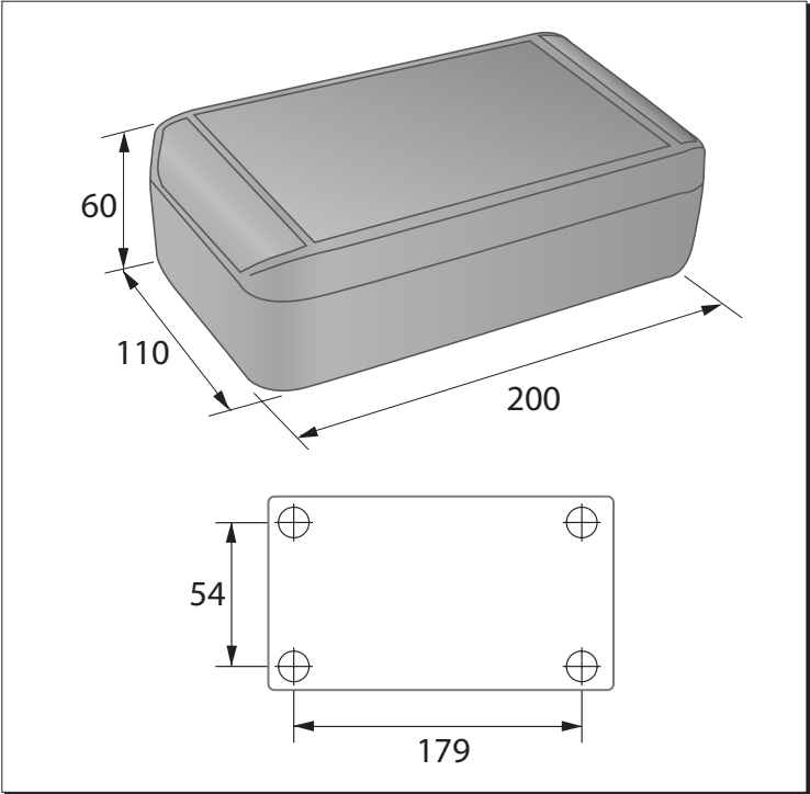
KS23 dimensions (Fig.4)
