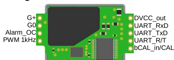
Figure 3. Attachment to customer's PCB, not in scale.
